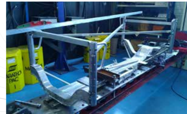
Scalp Trolley: 100% aluminum, bending & welding
